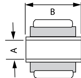
BUSHING & SLEEVE
